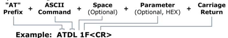
Figure B-14. Syntax for sending AT Commands
